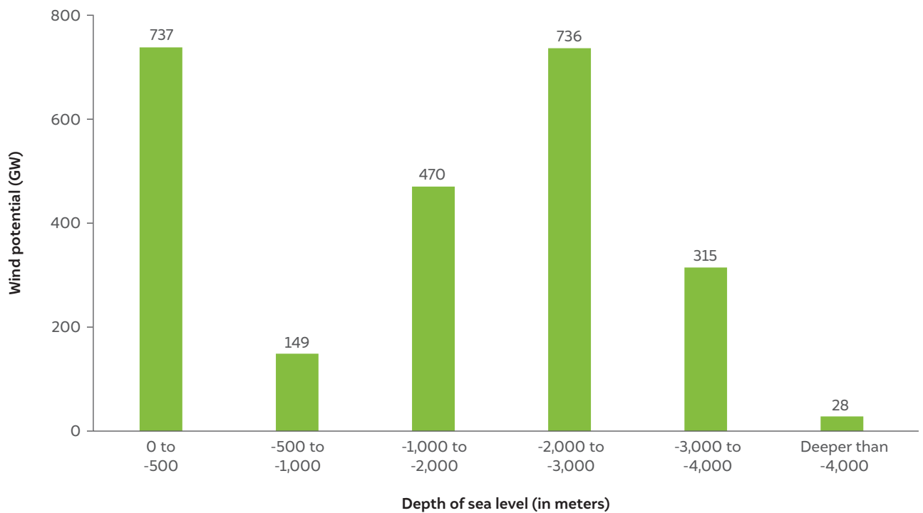
Figure 8 Only 30% of offshore wind potential is at depths less than 500 meters
