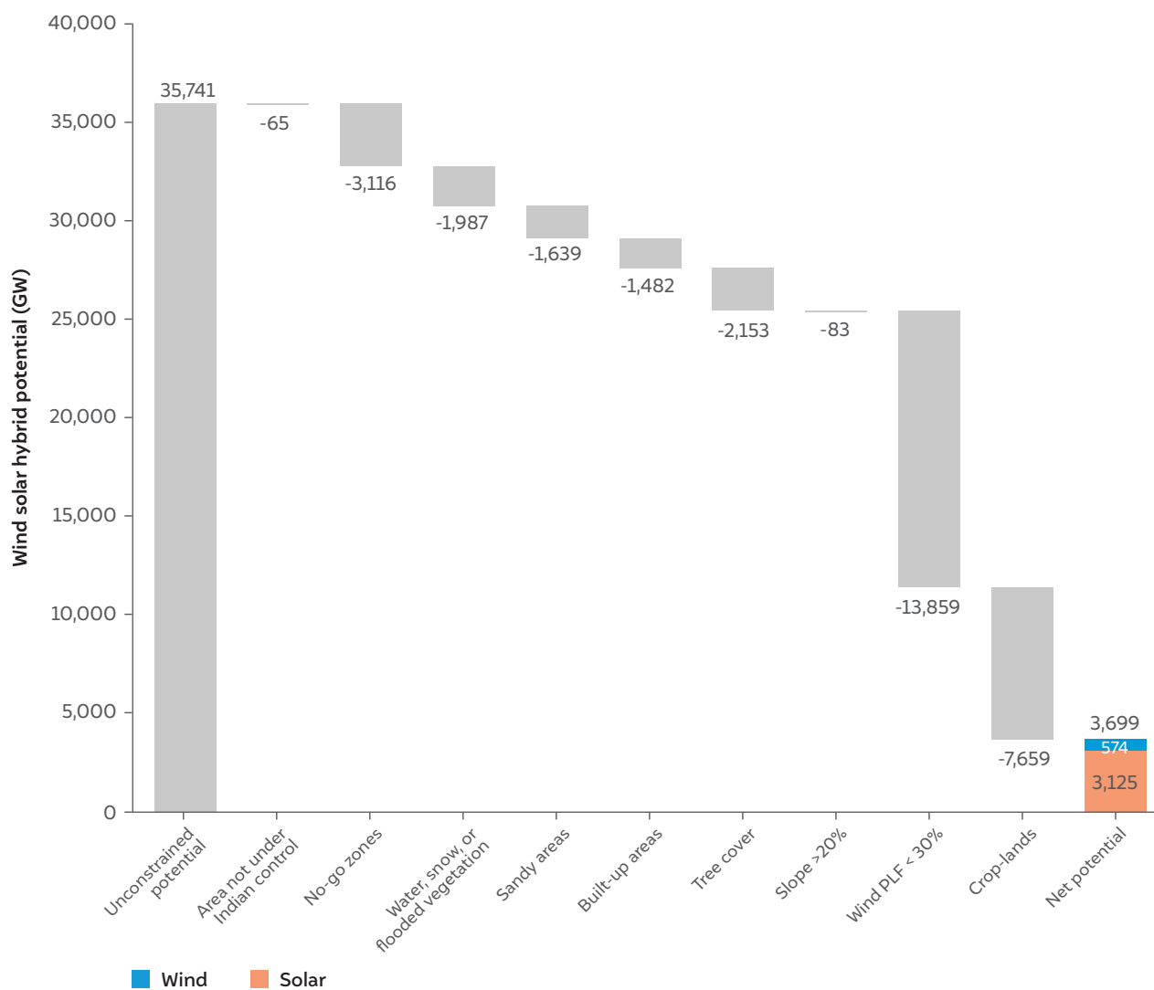
Figure 19 The co-located wind–solar hybrid potential in India is 3,699 GW but dominated mostly by 3,125 GW of solar power
