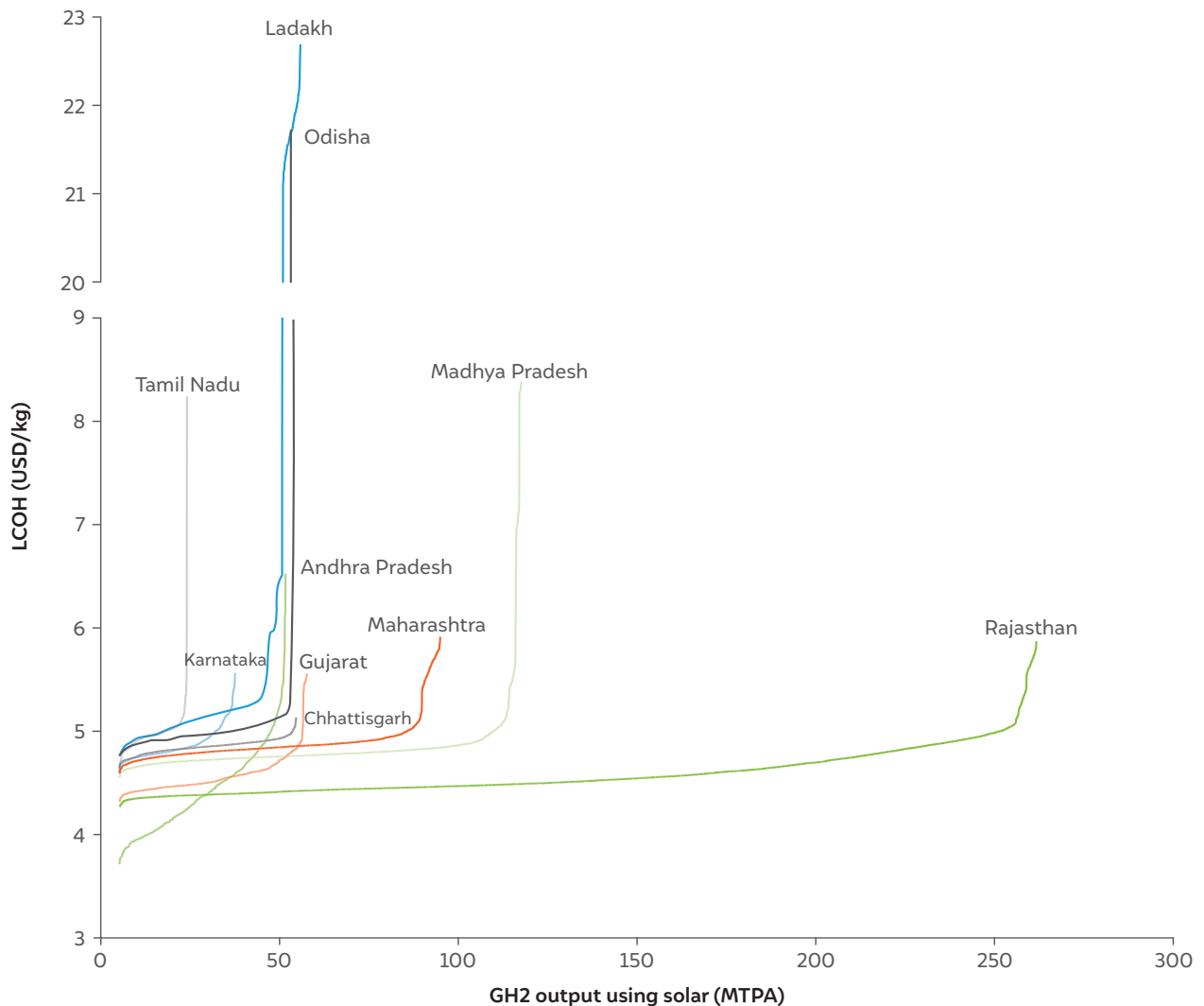
Figure 32 Rajasthan has the best solar resources for producing green hydrogen
