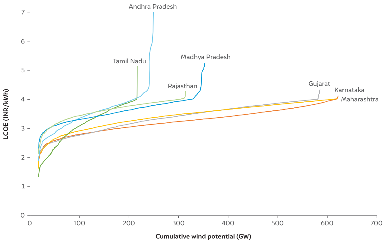
Figure 26 Karnataka, Gujarat, and Tamil Nadu have significant low-cost wind potential
