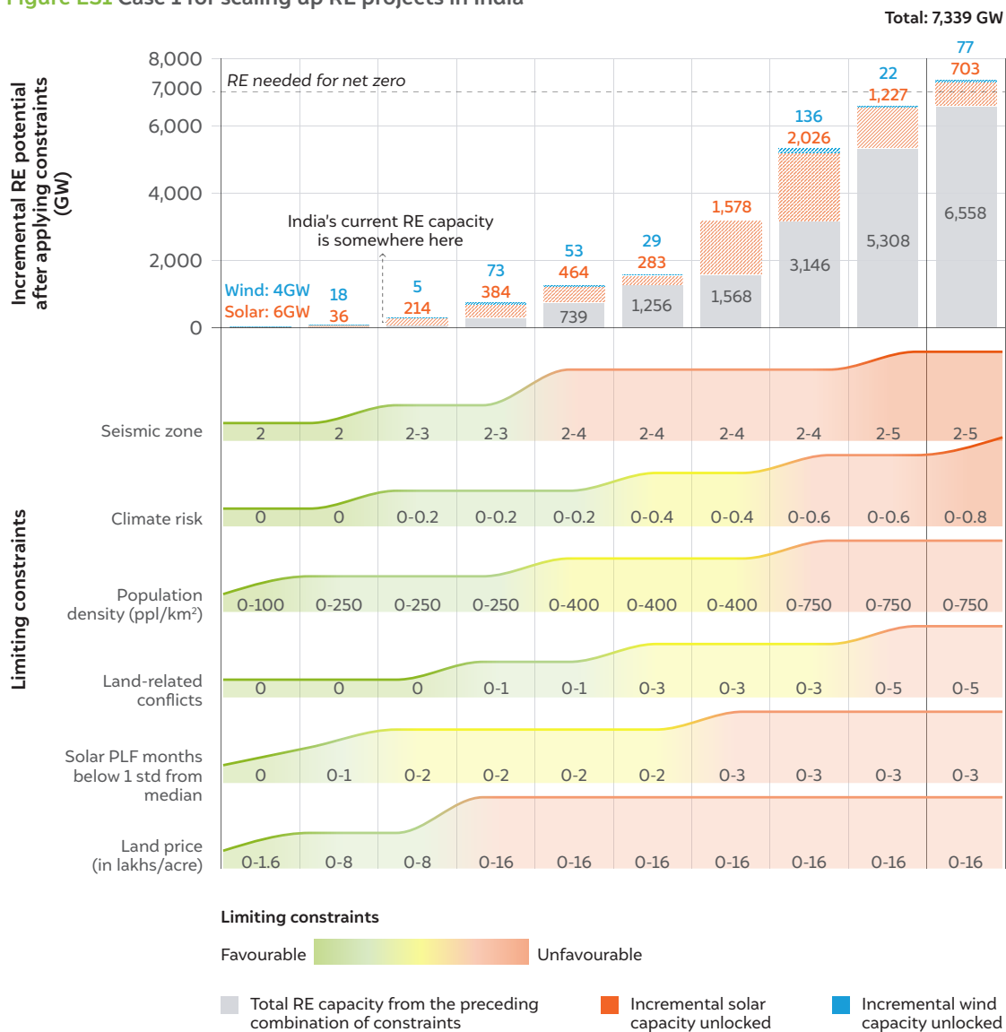
Figure ES1 Case 1 for scaling up RE projects in India
