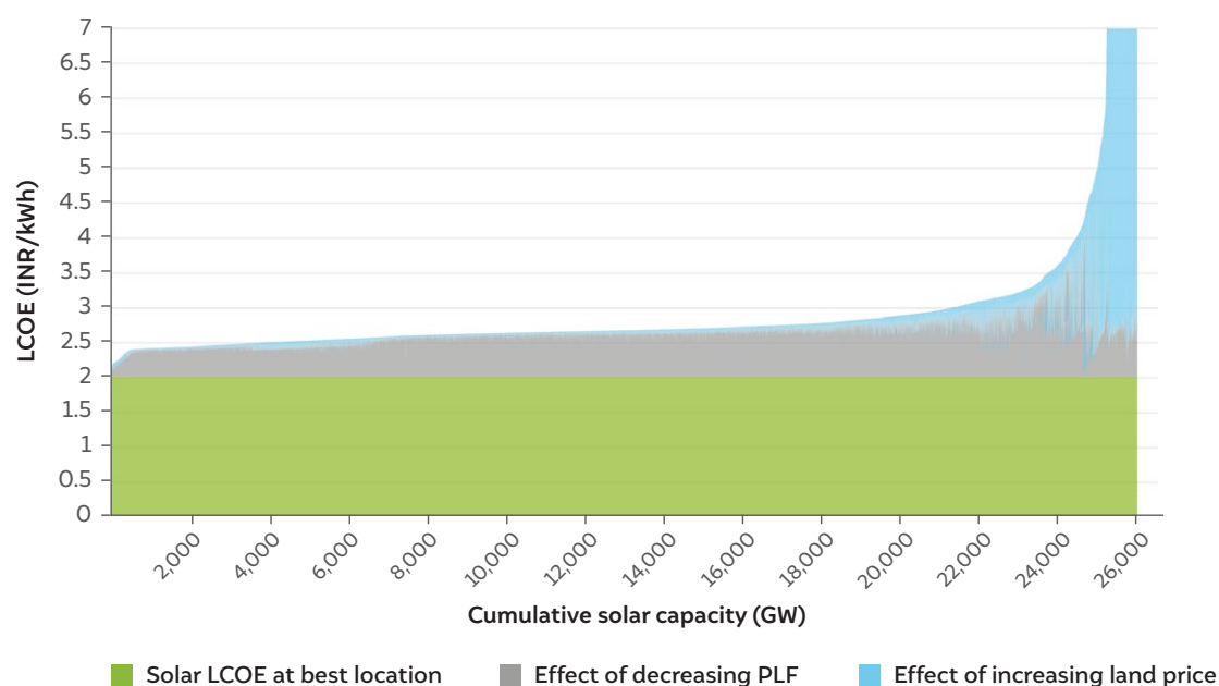
Figure 21 India has a solar potential of ~24,000 GW with a generation cost of less than INR 3 per kWh
