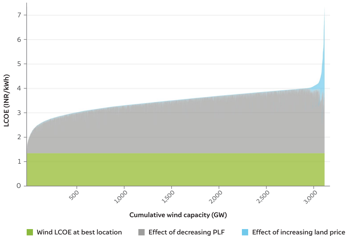
Figure 24 India has over 1,500 GW of wind potential at a generation cost less than INR 3/kWh
