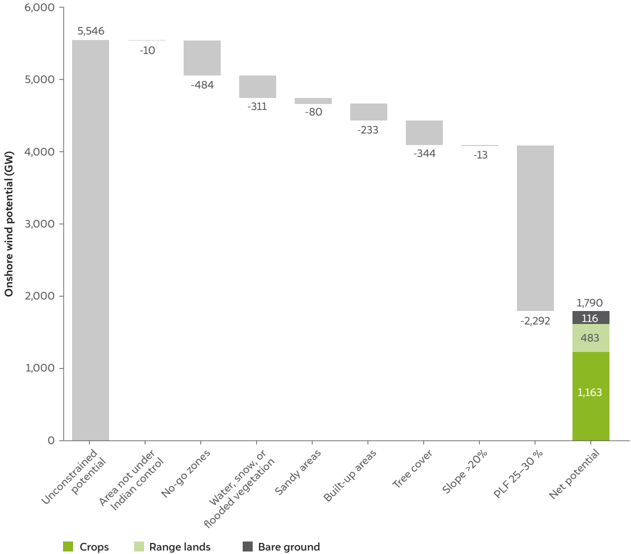
Figure 1 Wind potential in India is 1,790 GW
