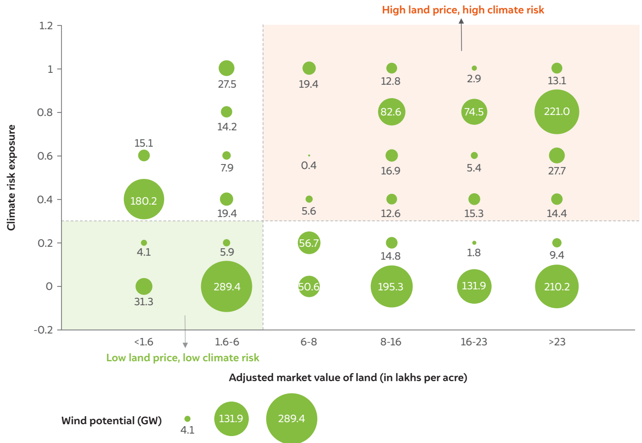
Figure 6 The wind potential, land prices, and climate risk exposure nexus indicate that 29% of the potential is in areas with both high land prices and high climate risk
