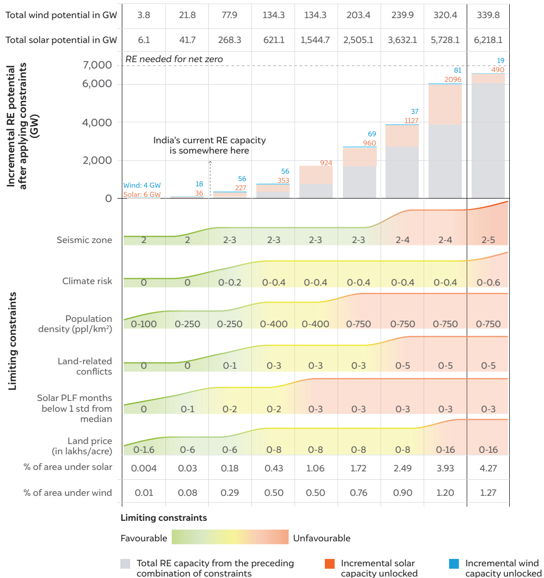
Figure 36 Case 2 for scaling up RE projects in India
