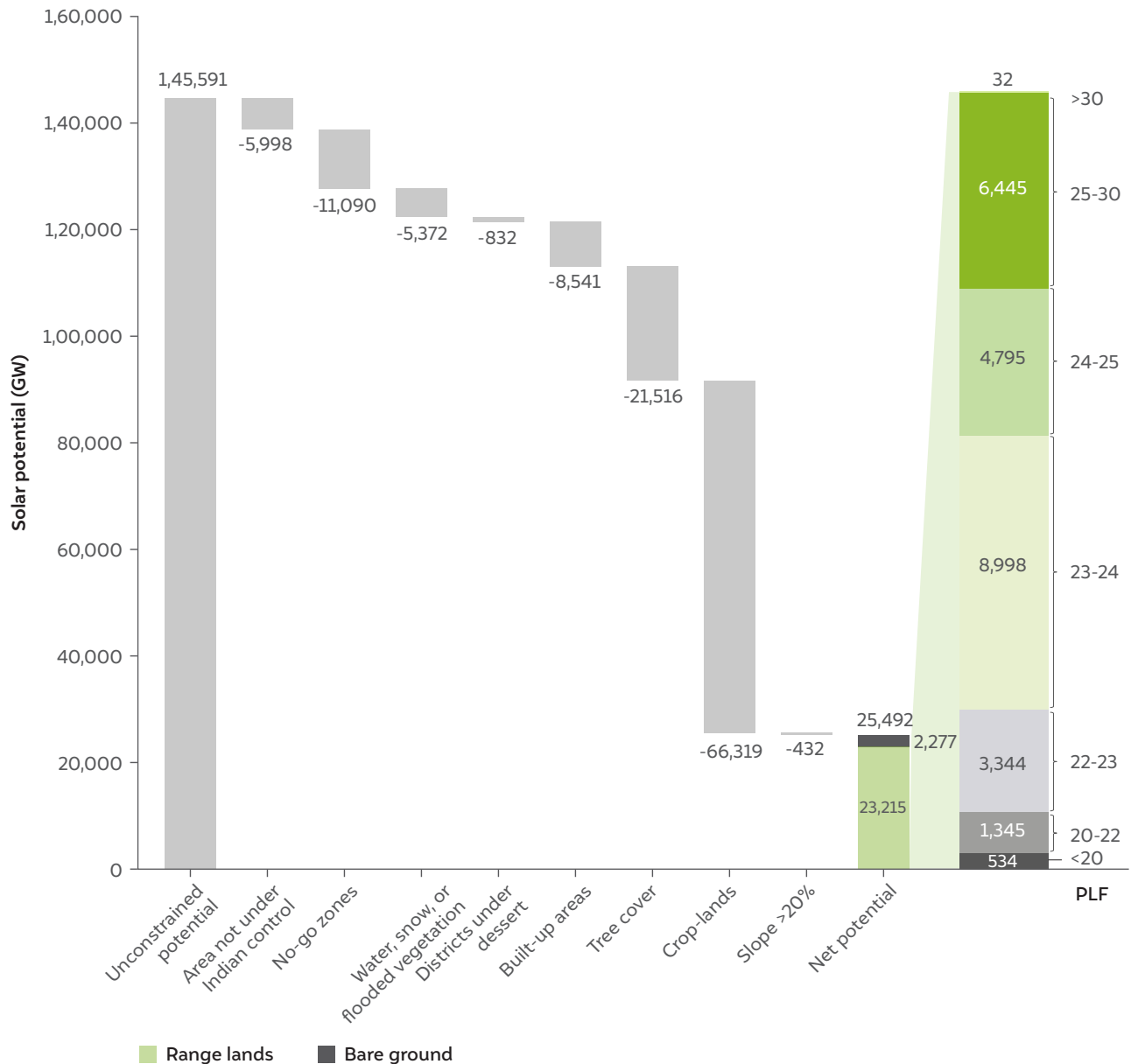
Figure 10 India has a solar potential of 20,270 GW with a PLF exceeding 23% (for 30% oversizing)
