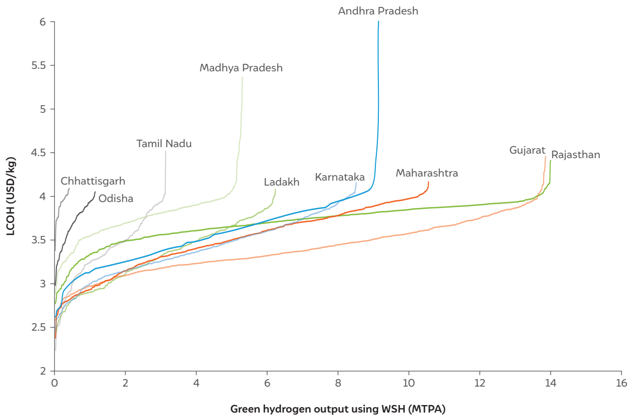
Figure 30 Gujarat, Karnataka, and Maharashtra have low-cost green hydrogen production potential
