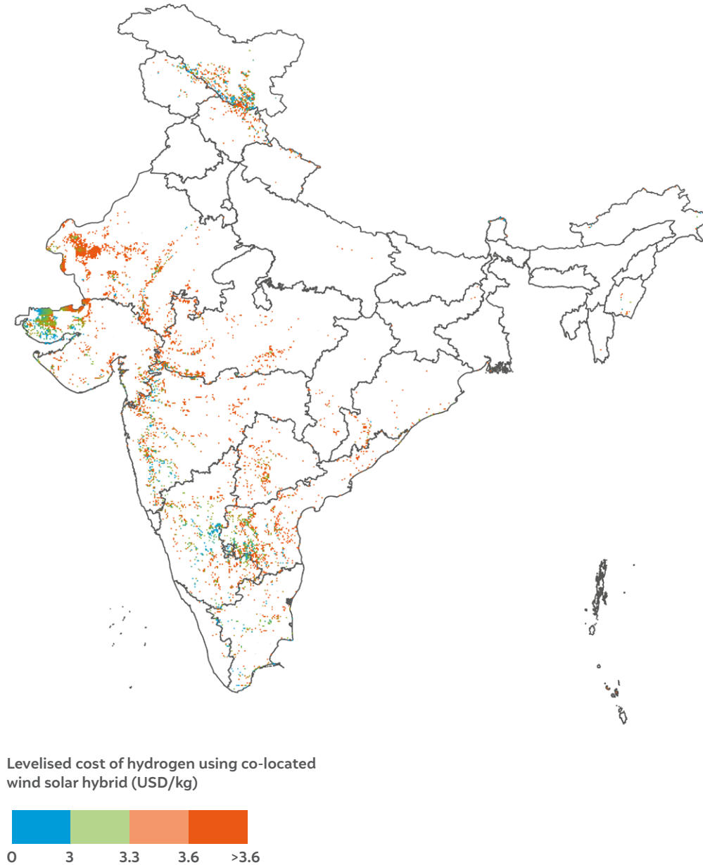
Figure 29 Low-cost green hydrogen can be produced in western and southern India
