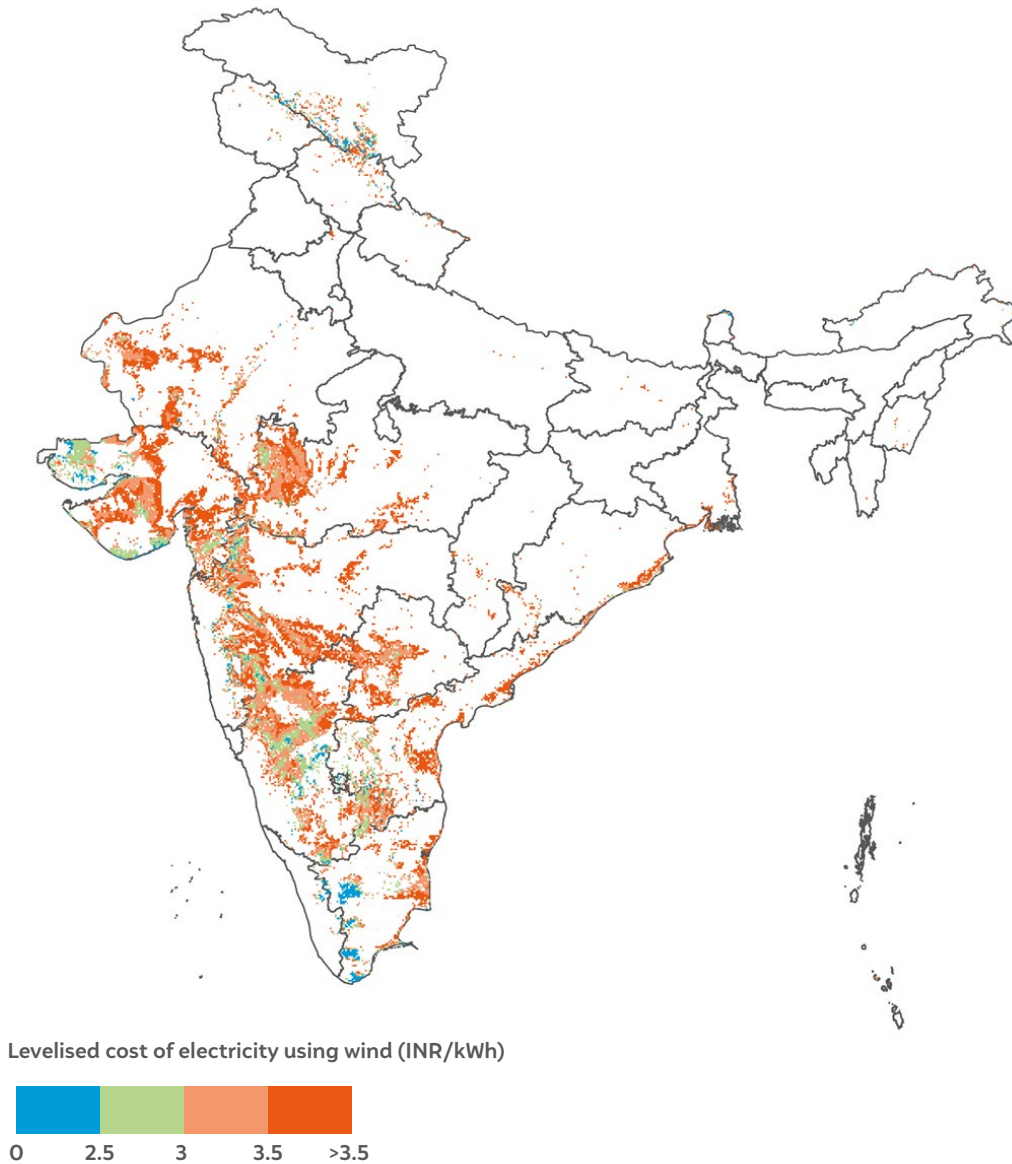
Figure 25 Only western and southern India have significant wind potential
