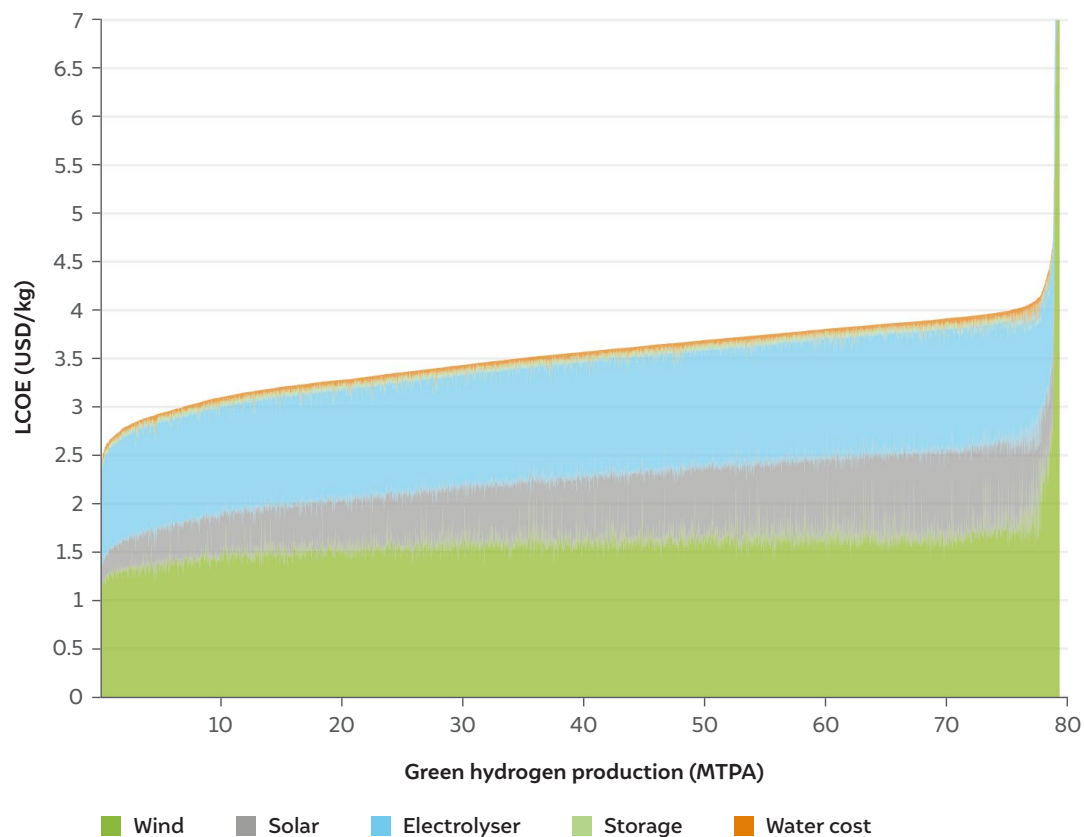
Figure 28 India can produce 40 MTPA of green hydrogen at costs lower than USD 3.5 per kilogram
