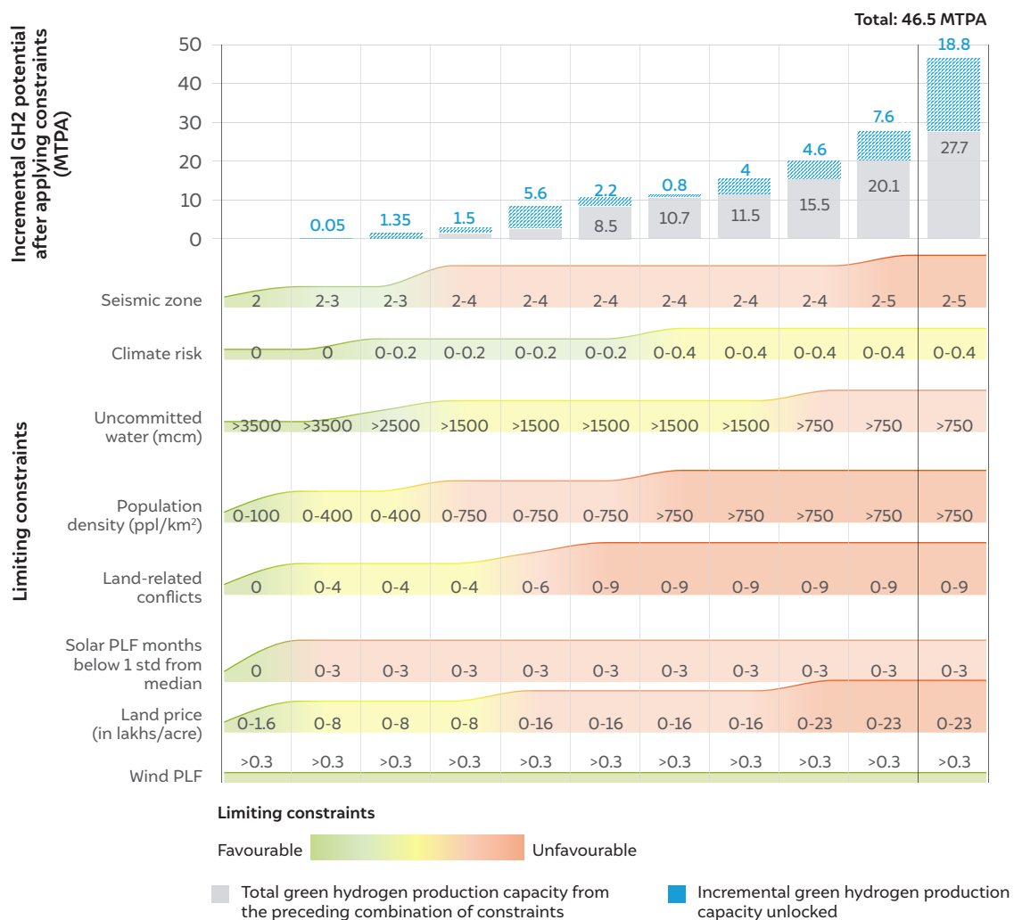
Figure ES3 Scaling up of green hydrogen projects in India will need overcoming multiple challenges
