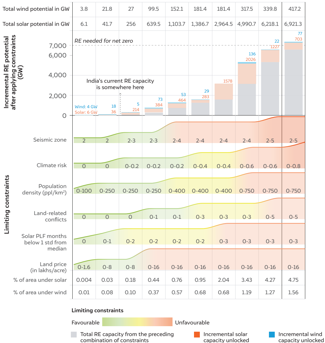
Figure 35 Case 1 for scaling up RE projects in India
