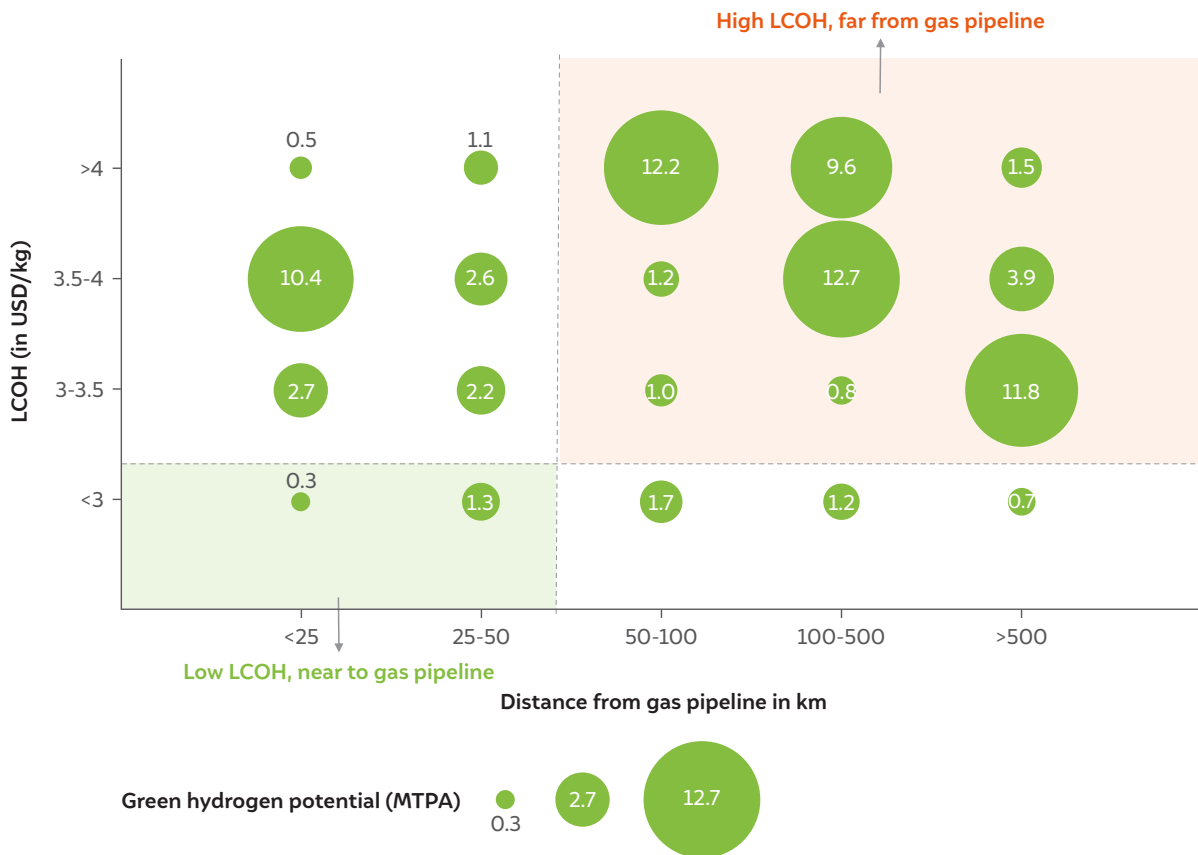
Figure 34 Only 1.6 MTPA of low-cost green hydrogen production potential is located within 50 kilometres of gas pipelines
