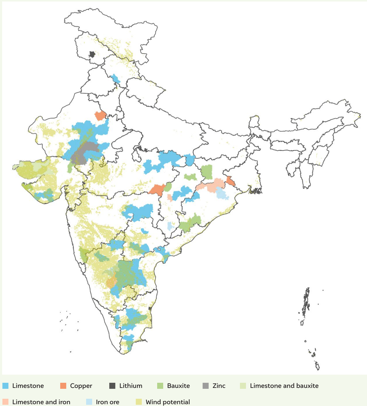
Figure 18 625 GW (35%) of wind potential is located in districts with mining activities
