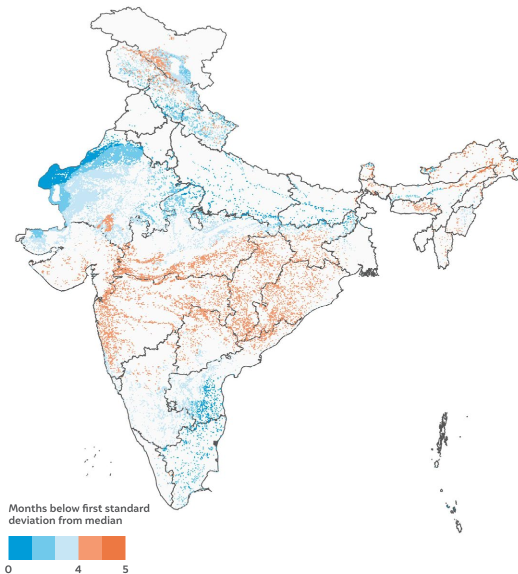
Figure 11 Most states in India have significant solar potential, but states like Maharashtra, Telangana, Chhattisgarh, and Odisha face high seasonality in solar PLF
