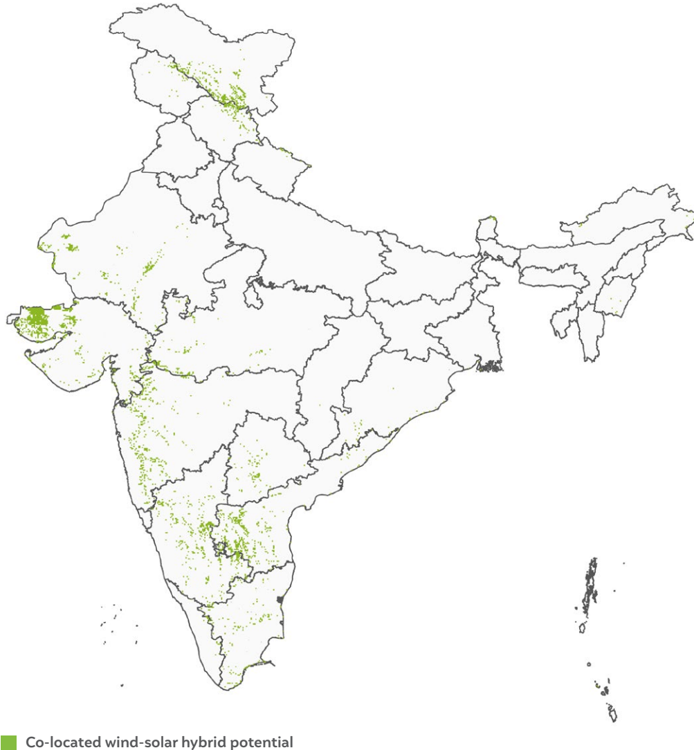
Figure 20 Wind–solar hybrid sites are located in the western and southern part of India
