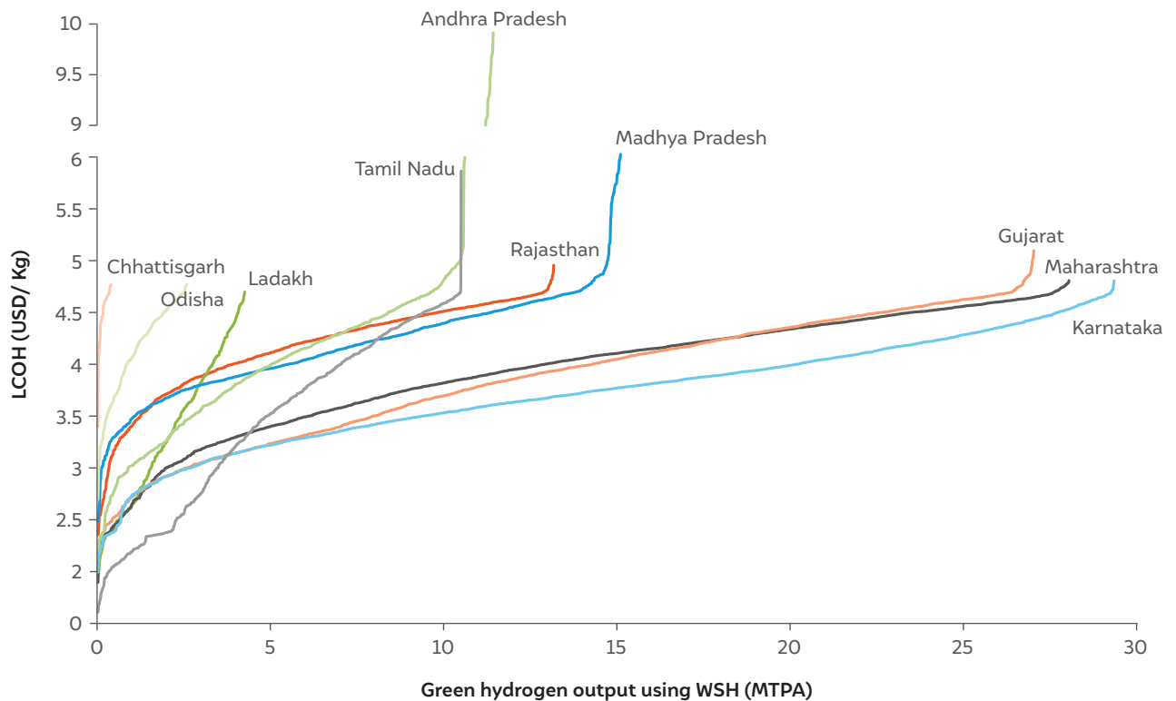
Figure 31 Tamil Nadu has the most favourable wind resources for producing low-cost green hydrogen
