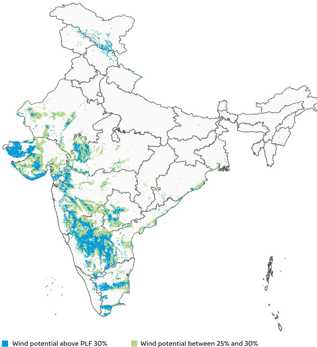
Figure 2 Onshore wind potential in India is concentrated in the western and southern parts
