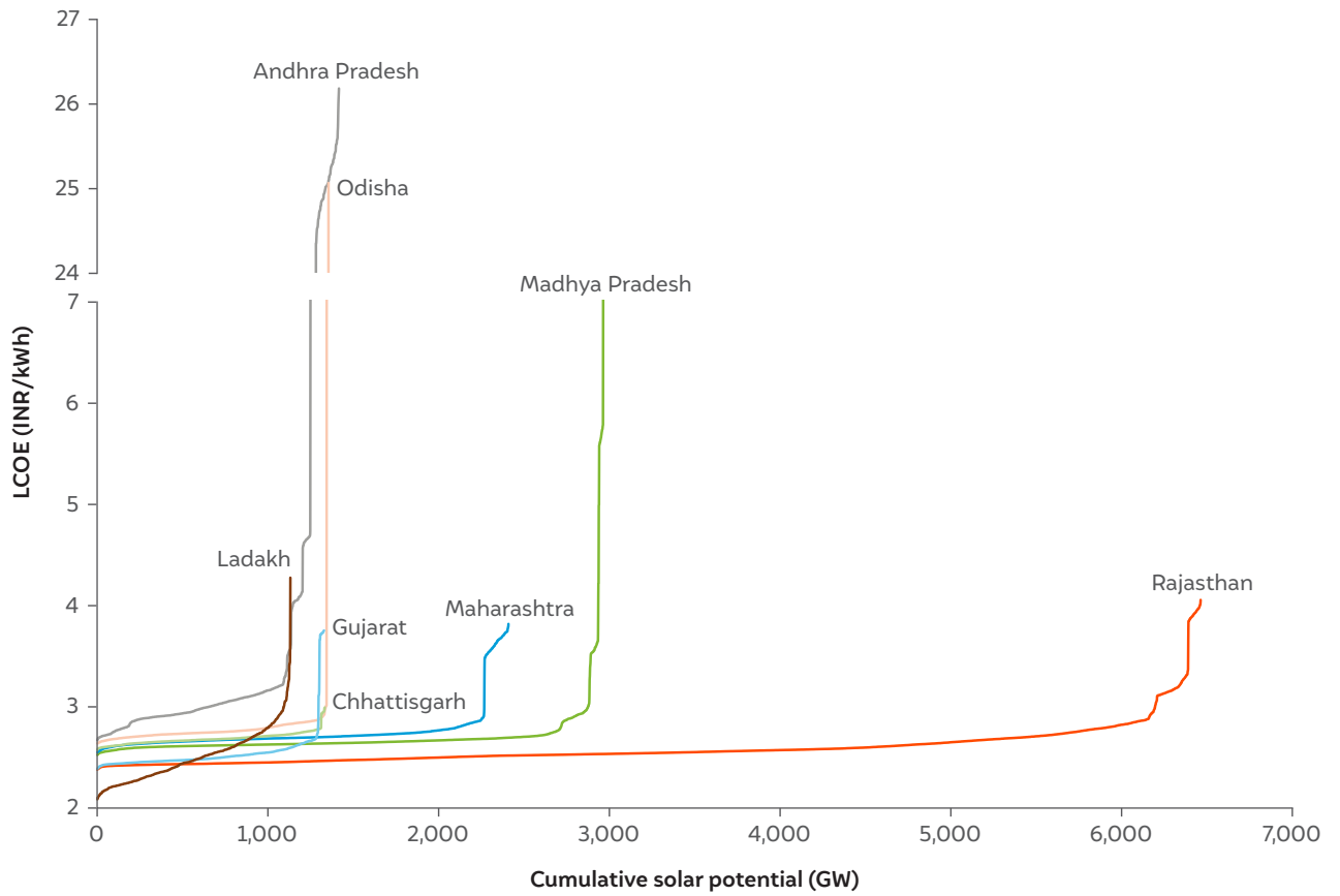
Figure 23 Rajasthan has the highest solar potential and the lowest generation cost
