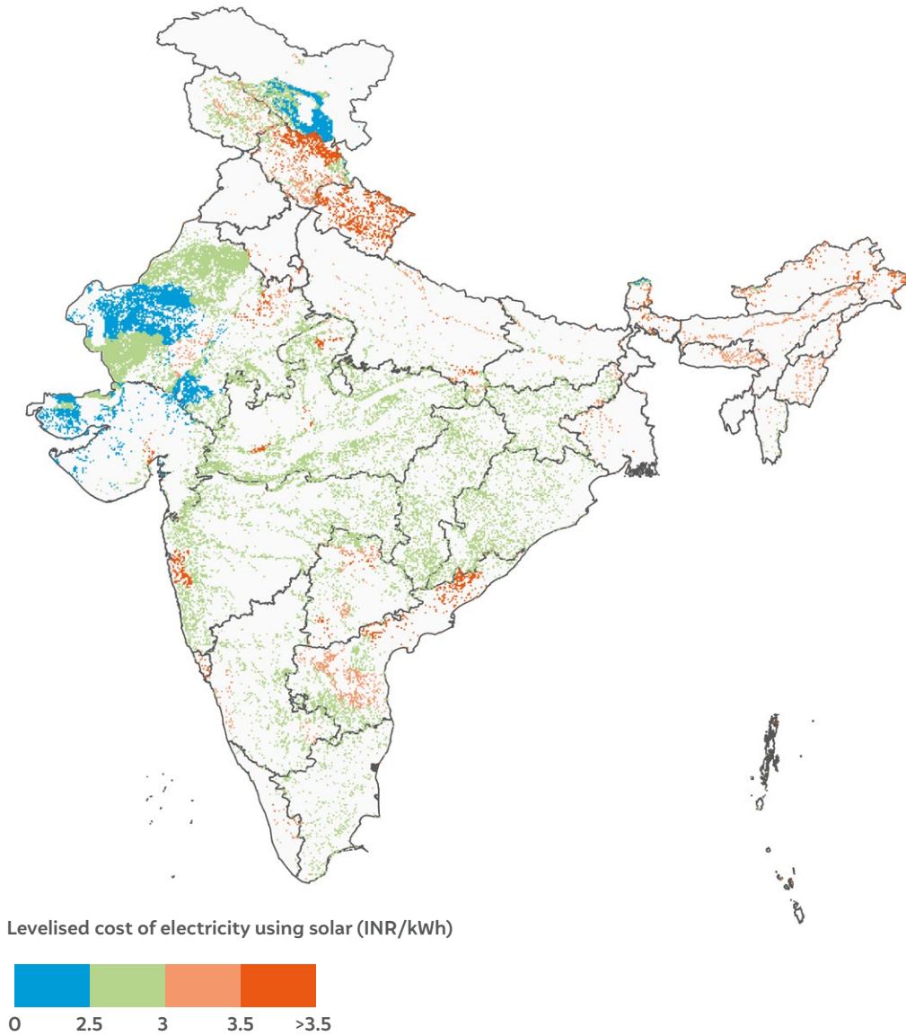
Figure 22 Western and central India have significantly lower LCOE compared to other parts of the country
