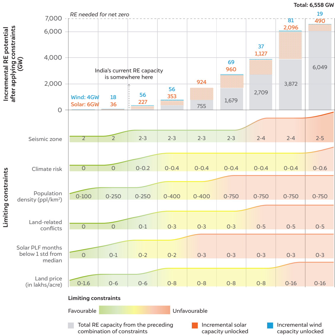
Figure ES2 Case 2 for scaling up RE projects in India
